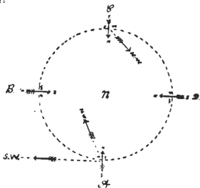
THE EARTH'S supposed ELLIPTICAL ORBIT
